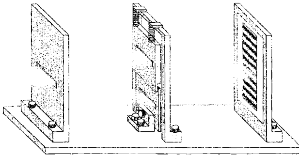
11 Bohr's two-slit interference device with a which-path detector. For details, see the caption for figure 6. From P. Bertet et al., "A Complementarity Experiment with an Interferometer at the Quantum-Classical Boundary," Nature 411 (2001): 167, figure 1. Reprinted with permission of Macmillan Publishers Ltd.
