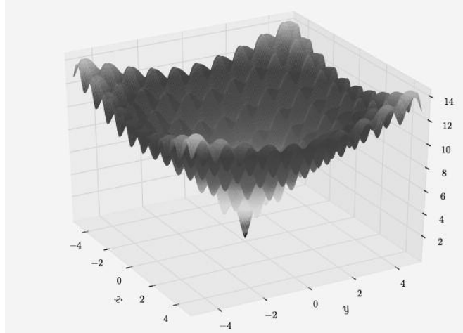
Ackley benchmark function. Image: Gaortiz, Wikimedia Commons.
